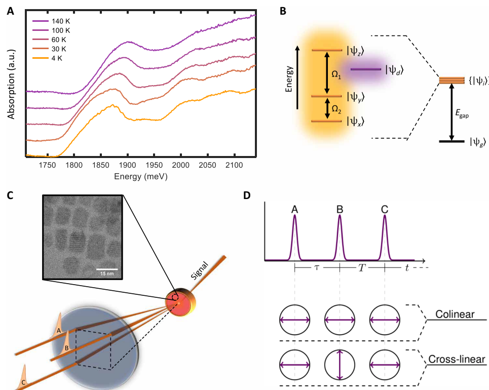
Fig. 1. CsPbI 3 perovskite NCs studied via MDCS. (A) Perovskite NC absorption spectra as a function of temperature (34). (B) Energy level diagram of the nondegenerate bright triplet states \{|\Psi_{x/y/z}\rangle\} that comprise the band-edge transitions to and from |\Psi_g\rangle . The dark singlet state |\Psi_d\rangle is shown to lie between states |\Psi_y\rangle and |\Psi_z\rangle , which is argued in the main text. (C) Schematic of the MDCS experiment. Three pulses {A,B,C} are focused onto the sample with varying time delays. Inset shows a transmission electron micrograph of representative CsPbI 3 NCs. (D) Excitation pulse sequence and excitation polarization schemes used to acquire one-quantum and zero-quantum spectra, in which double-sided arrows in circles denote the polarization of each pulse. Pulses A and C are horizontally polarized, and pulse B is either horizontally or vertically polarized, which corresponds to an emitted signal of either horizontal or vertical polarization respectively. a.u., arbitrary units.
